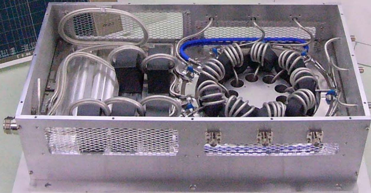
500kHz ~ 50MHz \geq 1000W , 9Way RF Broad Band Power Combiner
