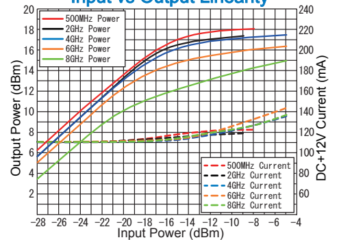
Input vs Output Linearity
