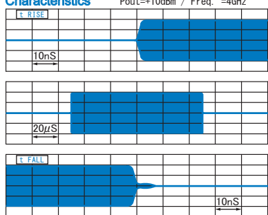
Pulse Characteristics
